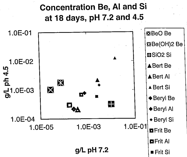
FIGURE 1. Concentration of Be, Al, or Si at 18 days, all materials pH 7.2 and 4.5.
