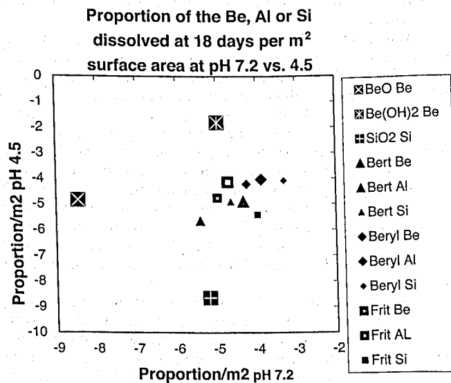
FIGURE 4. Proportion of Be, Al, or Si in solution at 18 days per sample surface area, at pH 7.2 and 4.5.
