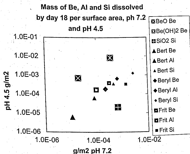
FIGURE 3. Concentration per sample surface area of Be, Al or Si at 18 days, at pH 7.2 and pH 4.5.
